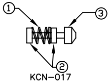
KCN-017 NEEDLE PACKING, COMPLETE, TEFLON GRAPHITE NEEDLE SHOWN FOR PLACEMENT OF PARTS
