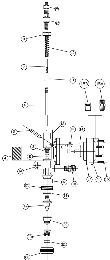
EXPLODED ASSEMBLY VIEW (SIDE)
